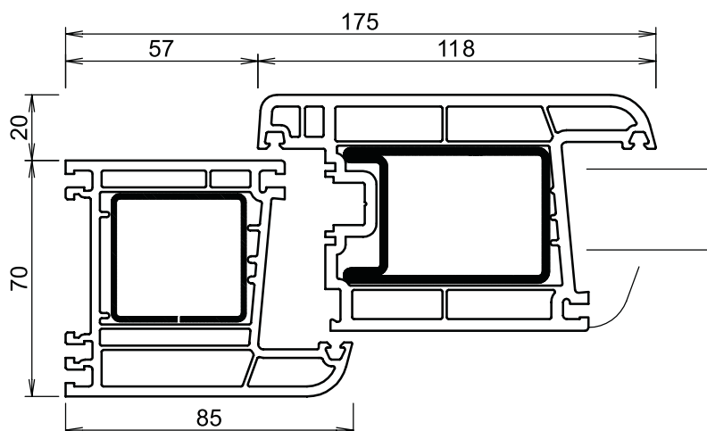
Marco F90-01-0102 Hoja F90-13-0115
