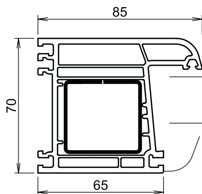
Marco F90-01-0102
