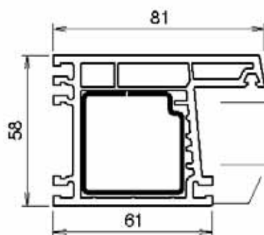
Marco F40-01-1402.W
